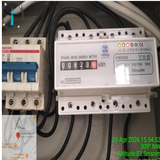
Counter Awal Kwh Meter
